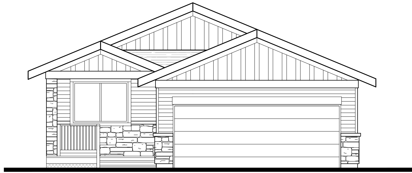
FRONT STREET ELEVATION
