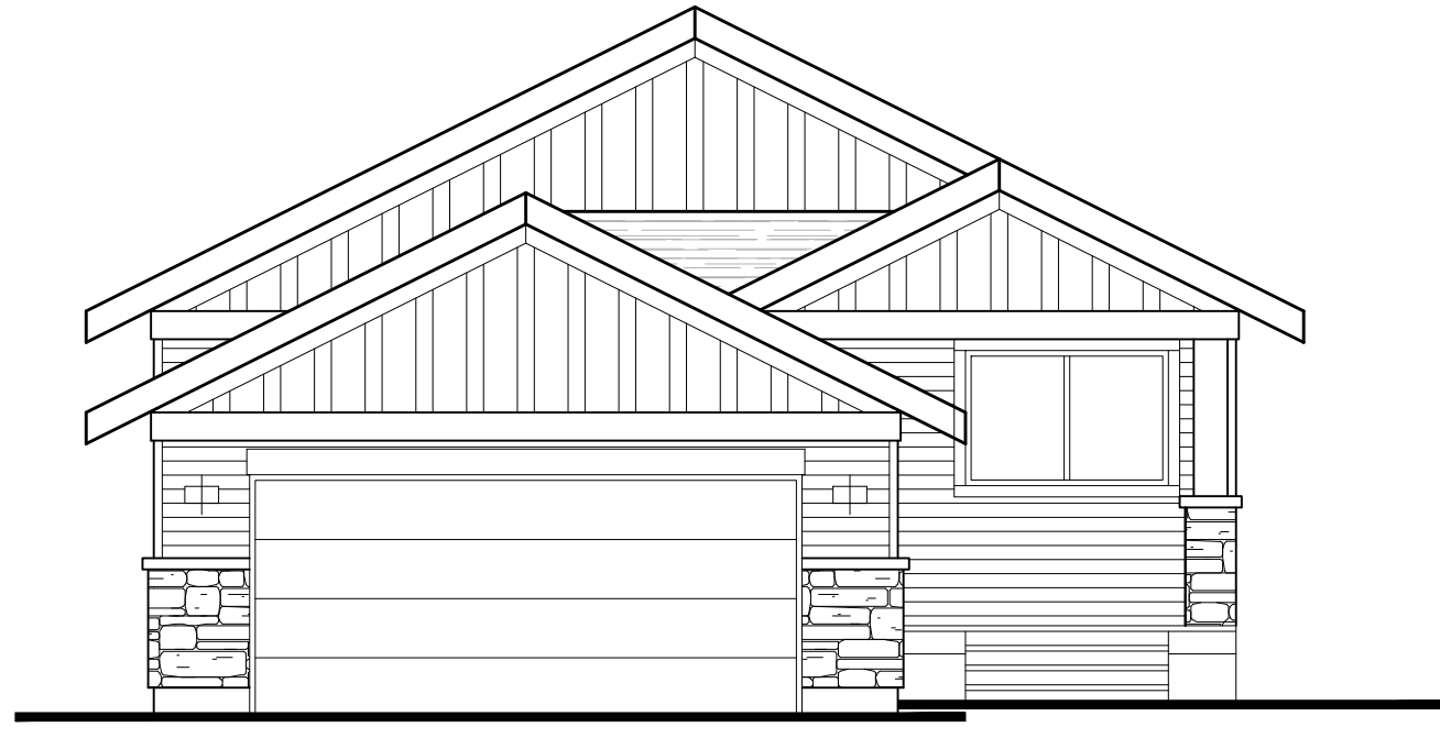
FRONT STREET ELEVATION
