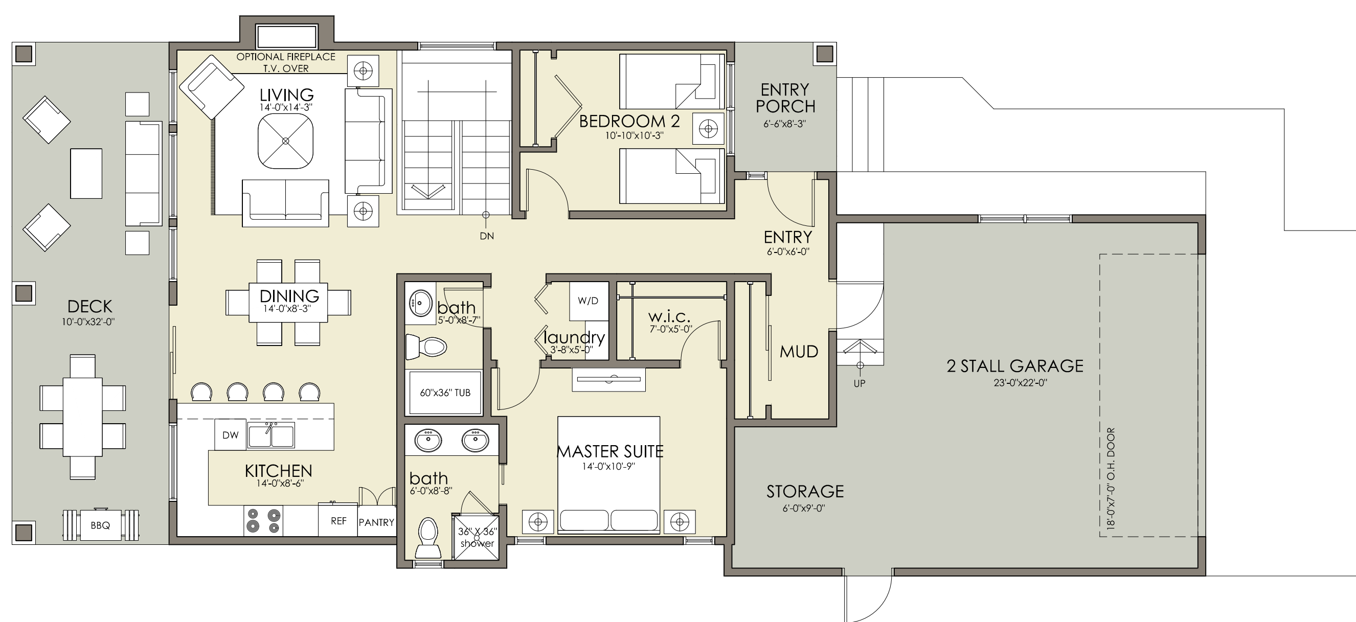
MAIN FLOOR PLAN 1268 SQ. FT. 2 BEDROOMS / 2 BATHS MAIN FLOOR LAUNDRY
